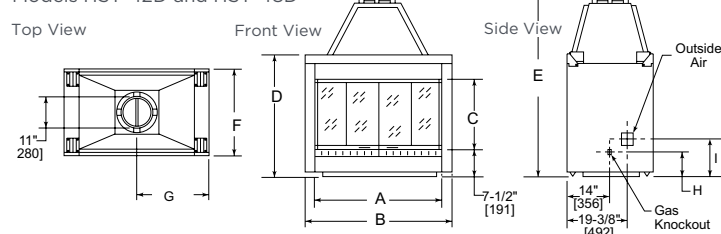
Models HST-42D and HST-48D
